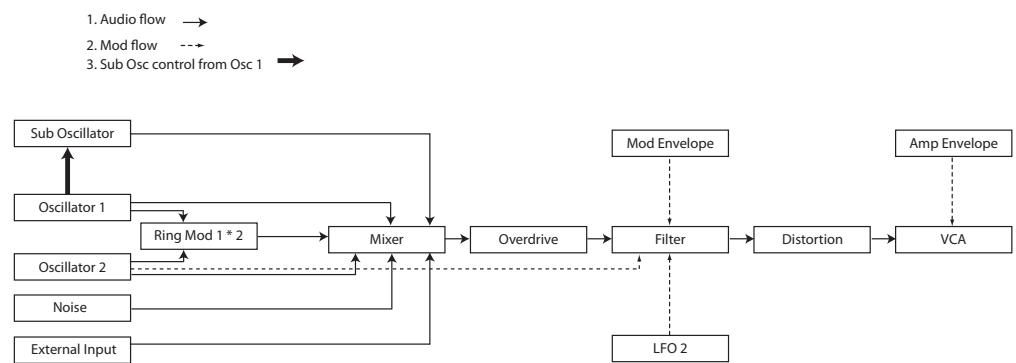
Bass Station II 模块图
